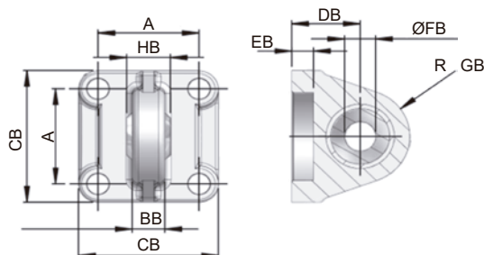
Charnela macho con rótula Single clevis with ball joint
