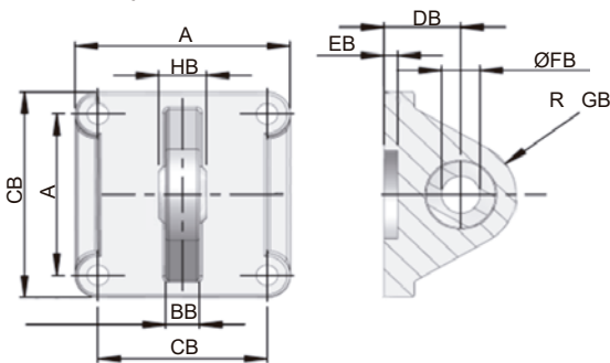
Charnela macho con rótula Single clevis with ball joint
